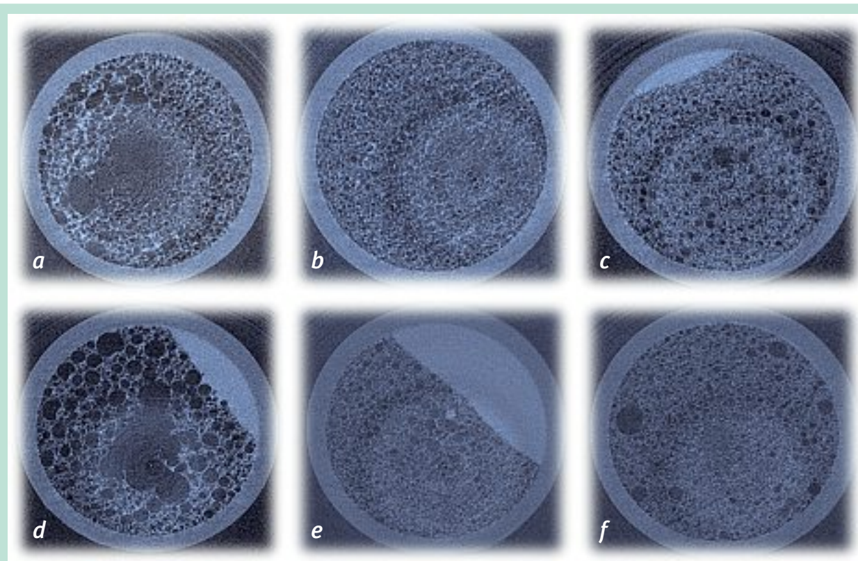
FIGURE 3 : Different foam structures obtained by varying the preparation parameters: (a) 3% 20 x C1; (b) 3% 20 x C1; (c) 0.5% 20 x C1; (d) 0.5% 50 x C1; (e) 0.5% 20 x C2; (f) 0.5% 50 x C2.
