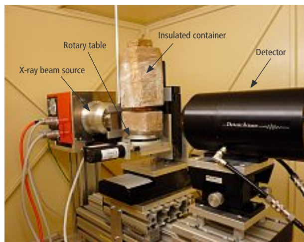
FIGURE 1 : The acquisition set-up at the Tomolab facility of Elettra (Trieste, Italy).
