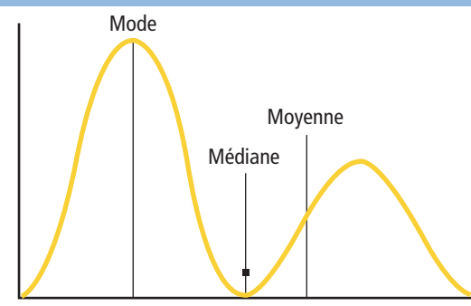
FIGURE 2 : Distribution polymodale.
