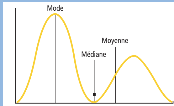
FIGURE 2 : Distribution polymodale.
