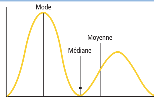
FIGURE 2 : Distribution polymodale.
