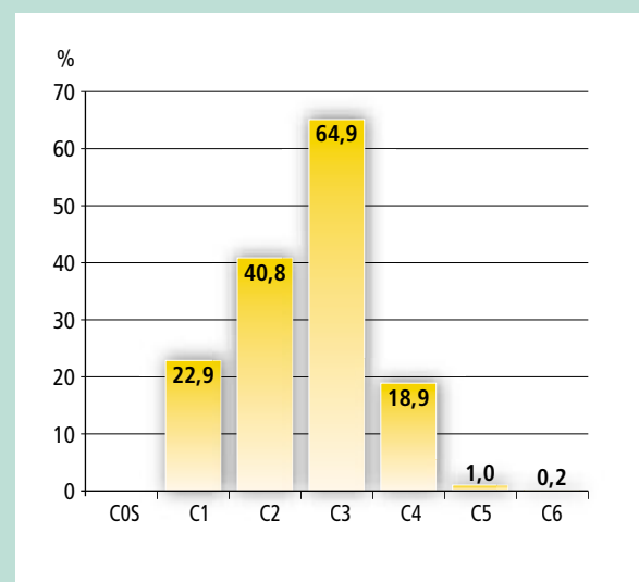
FIGURE 1 : Classification CEAP.
